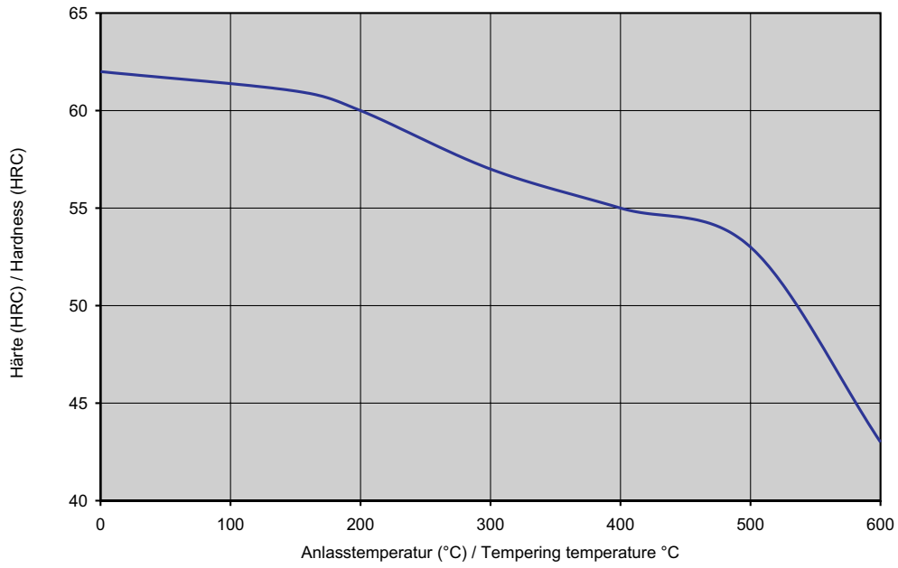
Tempering chart
